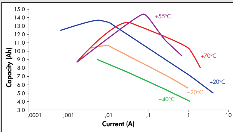
Capacity versus Current and Temperature (2.0 Volt cut off)
