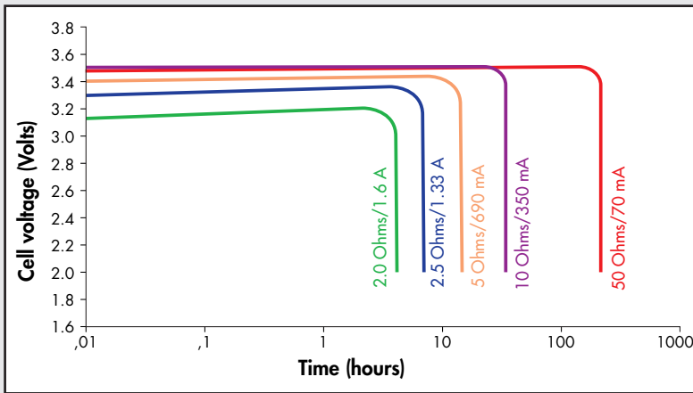
Discharge profiles at +55°C
